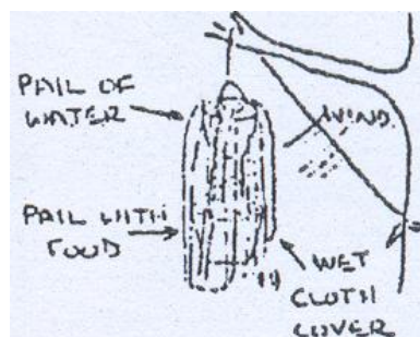
Evaporating cooler
